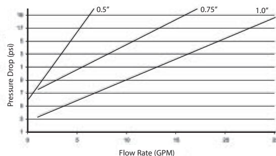
#34 Check Valves Pressure Drop vs. Flow 0.5"-1.0"
