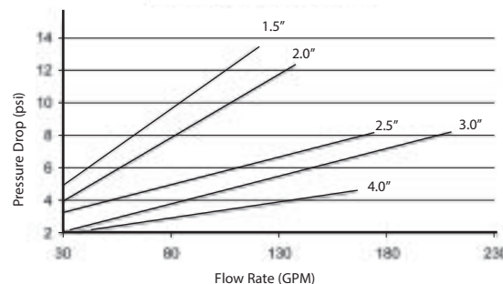
#34 Check Valves Pressure Drop vs. Flow 1.5"-4.0"
