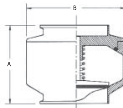
#34 Disc Check Valve
